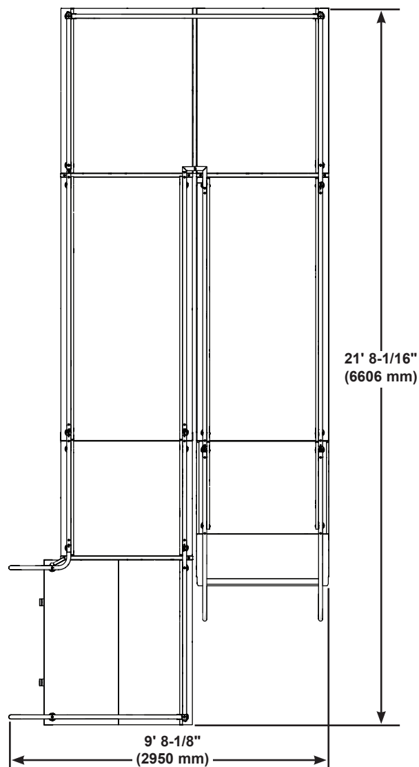
282A020 - 24" (610 mm) Elevation with Left Hand Switch and Right Hand Landing
