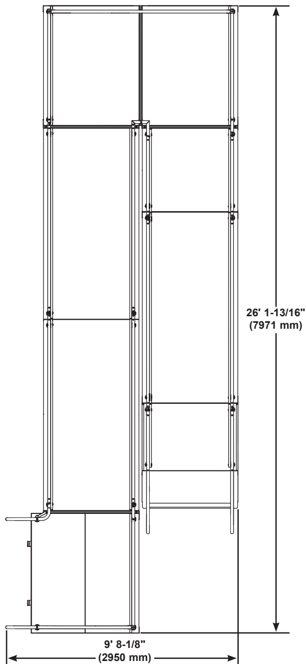
282A025 - 32" (813 mm) Elevation with Left Hand Switch and Right Hand Landing
