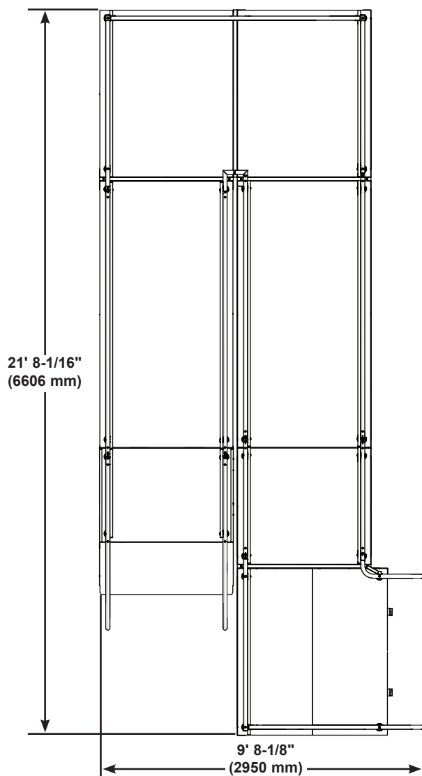
282A019 - 24" (610 mm) Elevation with Right Hand Switch and Left Hand Landing
