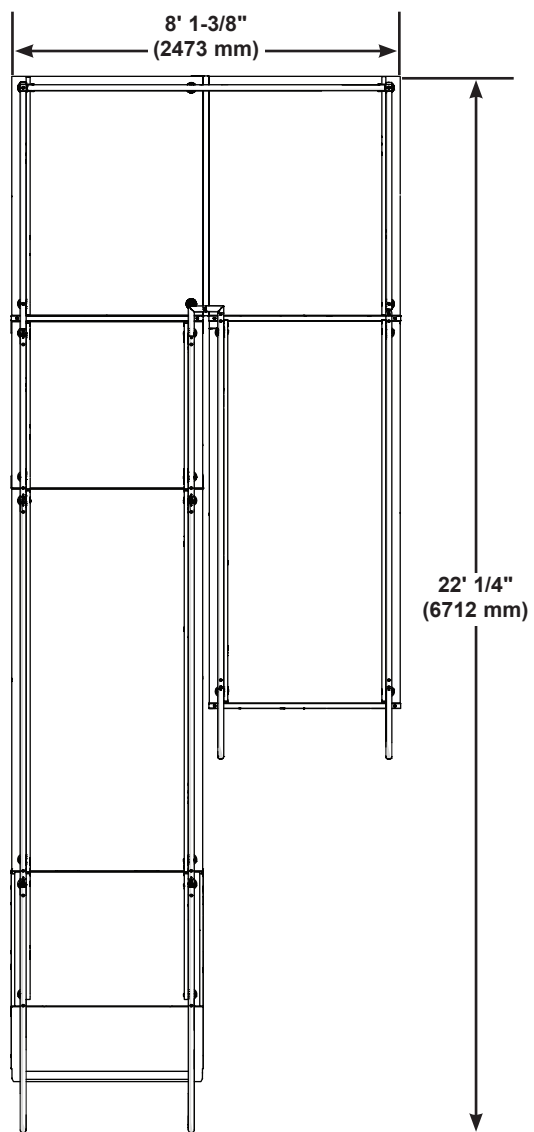
282A018 - 24" (610 mm) Elevation with Right Hand Switch
