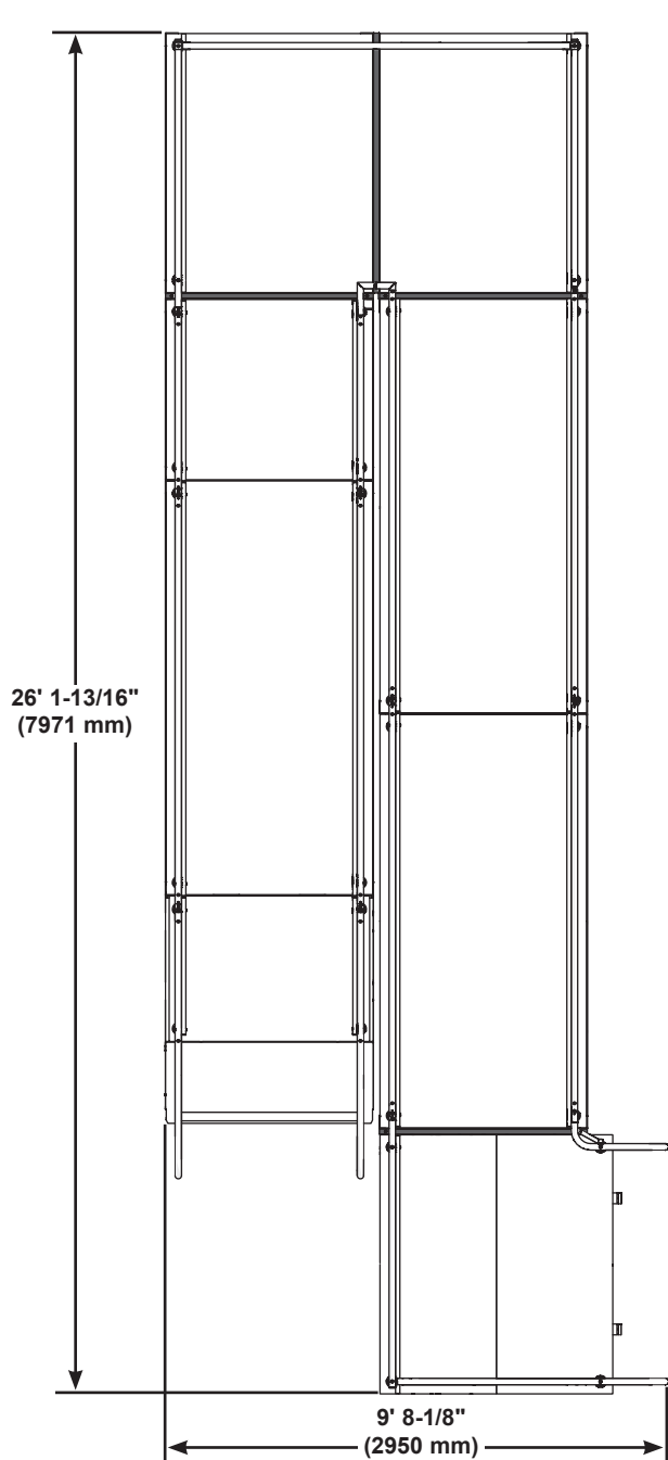
282A024 - 32" (813 mm) Elevation with Right Hand Switch and Left Hand Landing
